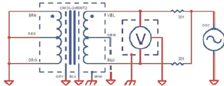
TEST CIRCUIT 3
